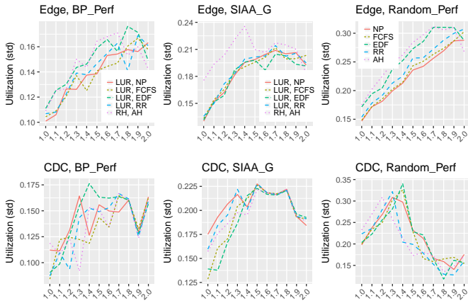
Fig. 14. Standard deviation of utilization of runtimes as node speed increases ( \gamma = 0.1 )
