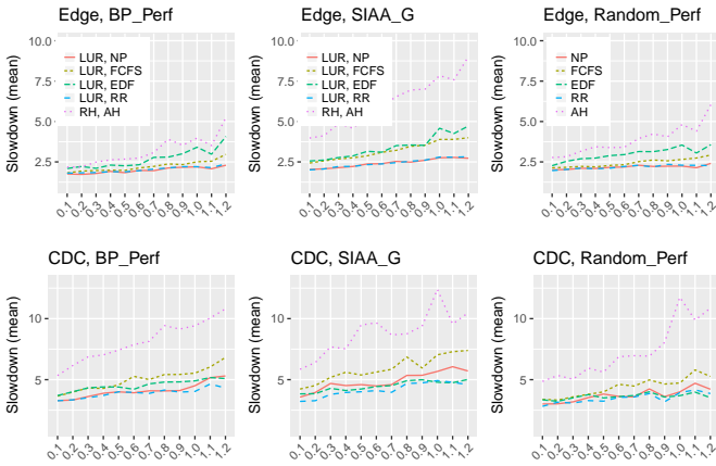
Fig. 6. Mean slowdown of applications as service time varies
