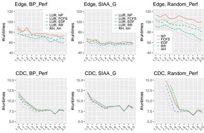
Fig. 10. For \gamma = 0.1 , mean number of runtimes as node speed increases
