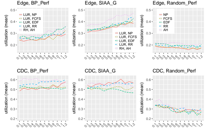
Fig. 8. Mean utilization of runtimes as service time varies
