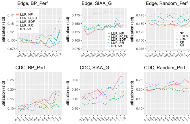
Fig. 9. Standard deviation of utilization of runtimes as service time varies
