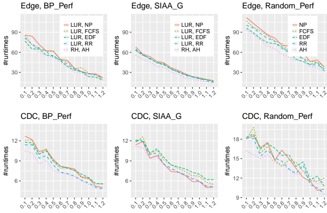
Fig. 5. Mean number of runtimes as service time varies
