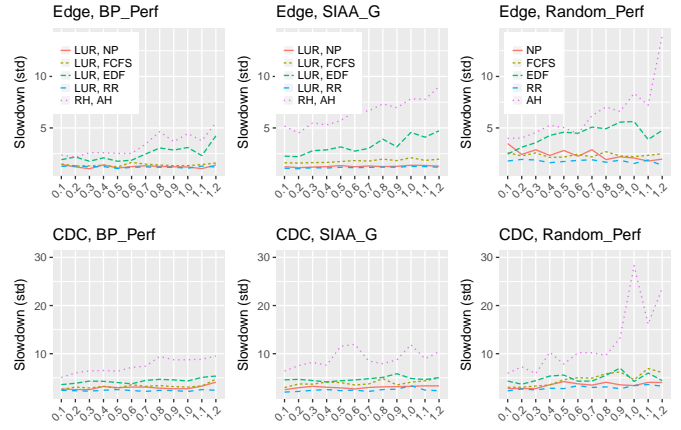
Fig. 7. Standard deviation of slowdown as service time varies
