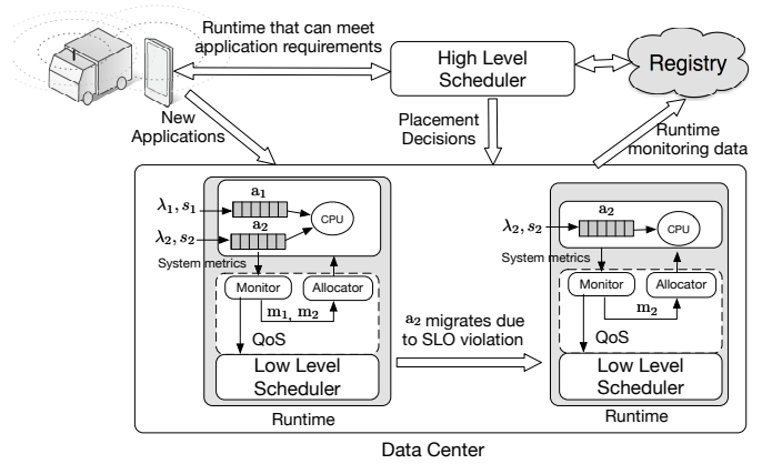
Fig. 4. Two-level scheduler for application placement in Mobile Edge Clouds
