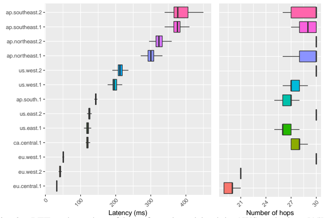
Fig. 2. RTT and number of hops for selected lambda AWS endpoints [15] from Umeå University.
