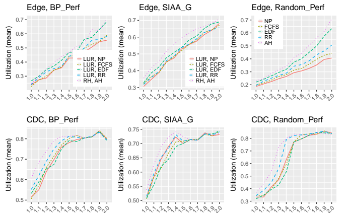
Fig. 13. Mean utilization of runtimes as node speed increases and \gamma = 0.1
