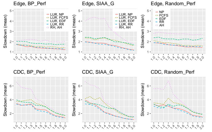
Fig. 11. For \gamma = 0.1 , mean slowdown as node speed increases
