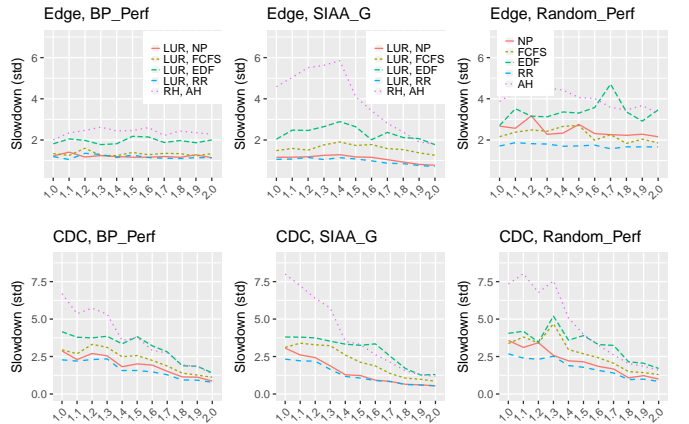
Fig. 12. Standard deviation of slowdown as node speed increases and \gamma = 0.1
